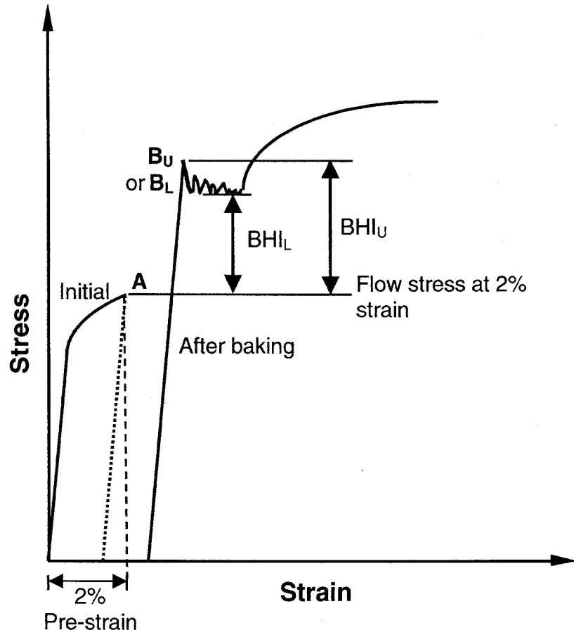
FIG. A1.1 Representation of Bake Hardening Index
